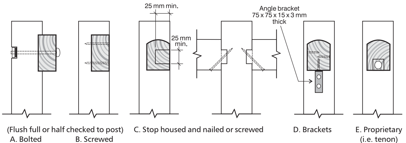
Figure 4. Handrail Connections
